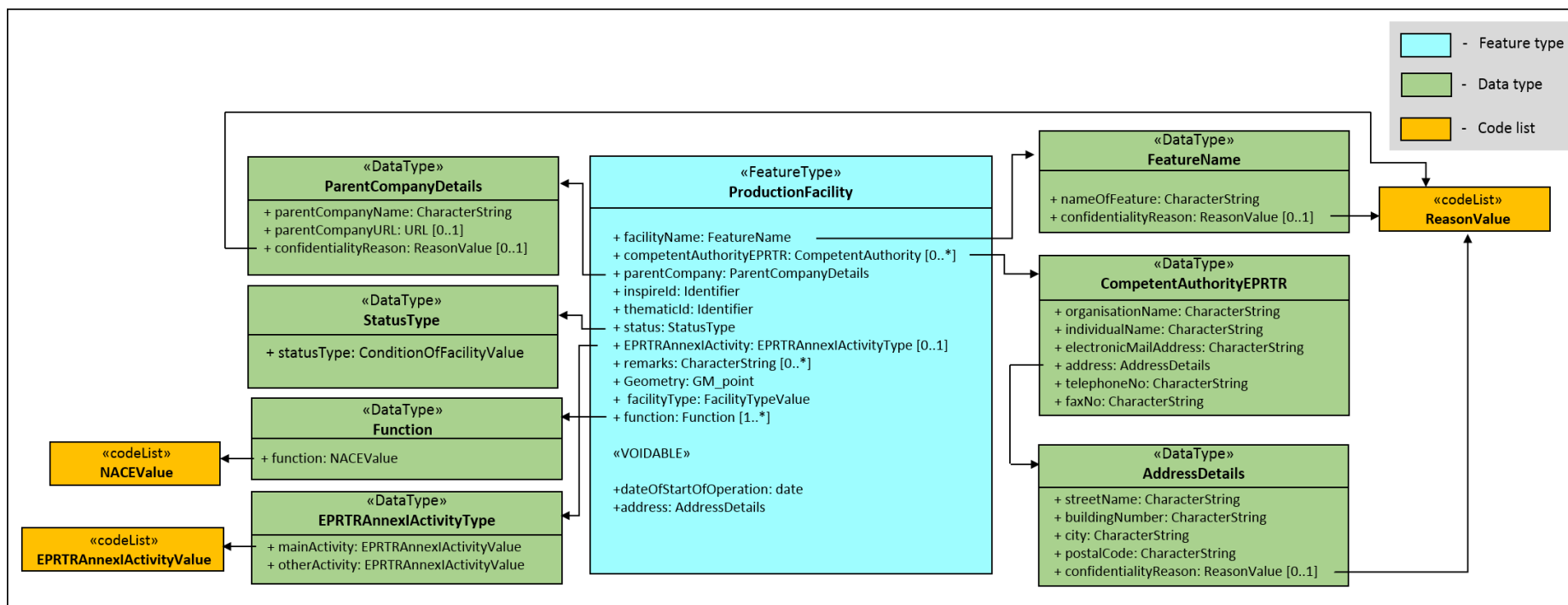
Figure 10 - ProductionFacility feature type, alongside connected data types and code lists.
