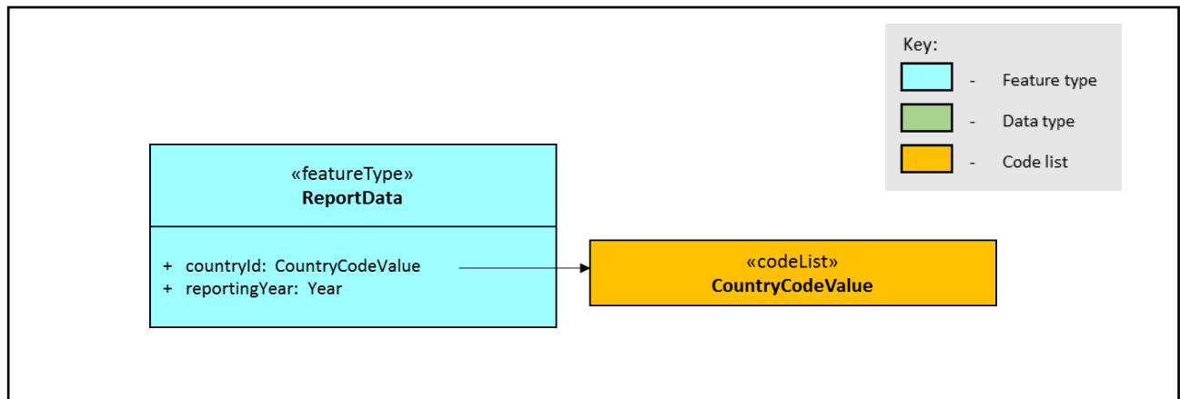
Figure 8 - ReportData feature type, alongside connected code list.
