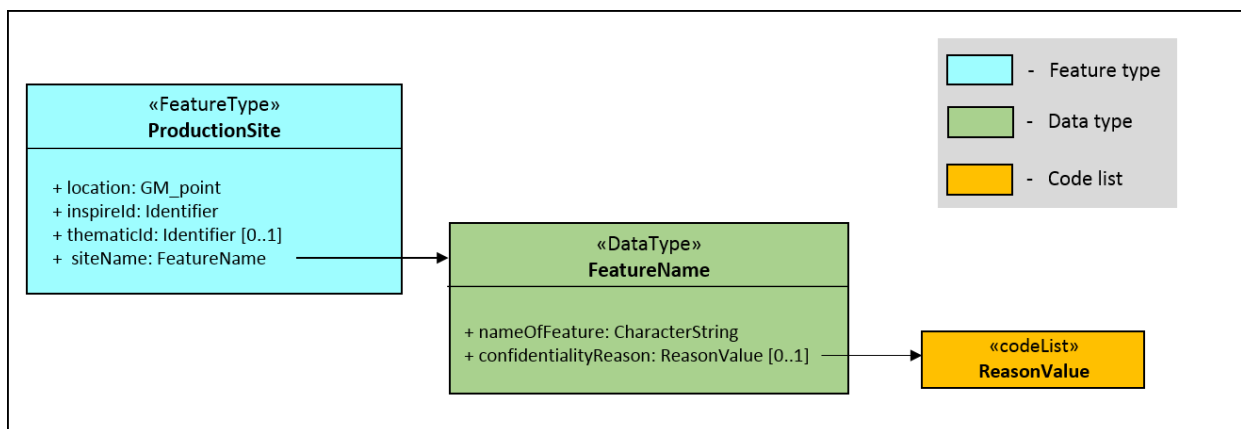
Figure 9 - ProductionSite feature type, alongside connected data types and code lists.
