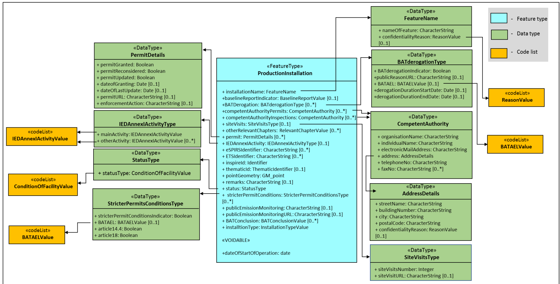
Figure 11 - ProductionInstallation feature type alongside connected data types and code lists.
