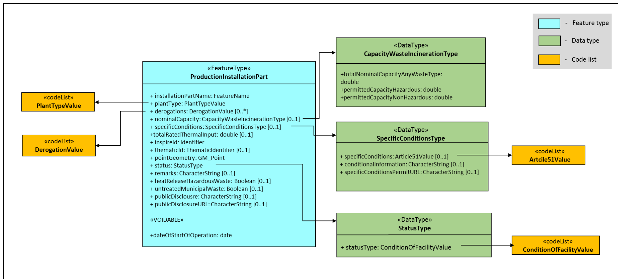
Figure 12 - ProductionInstallationPart feature type, alongside connected data types and code lists.
